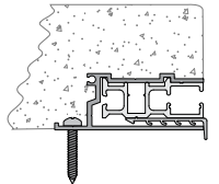
Undertrack with Dual-Race track channel
